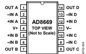
Figure 4. 14-Lead SOIC (R-14)
